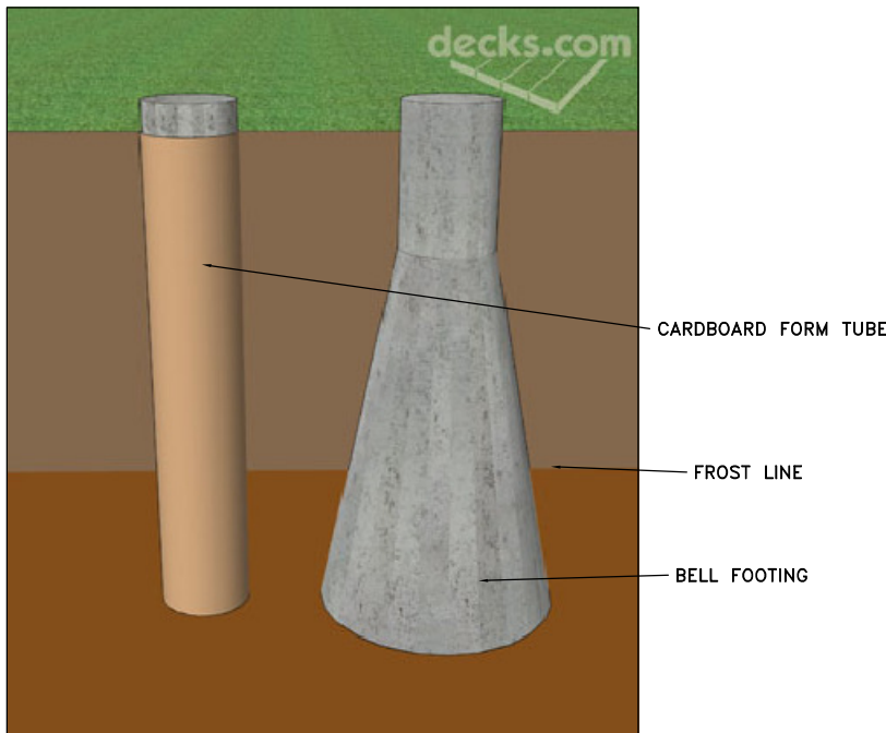
CONCRETE PIER FOOTING TYPE
