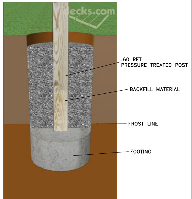
EMBEDDED WOOD POST FOOTING TYPE
