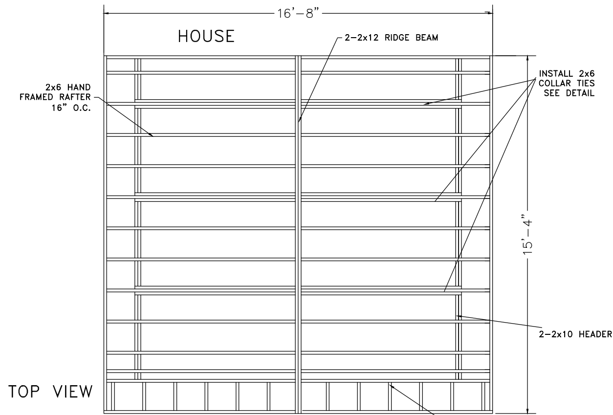
SECTION VIEW
